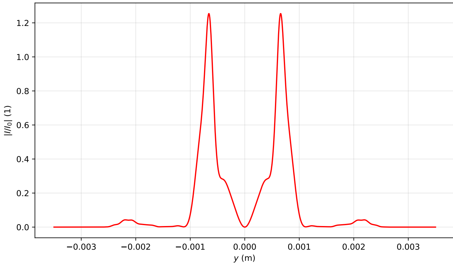
Intensity profile I(x=0, y, z=1.353)/I_0 , P_{in}=19.0P_{cr} , artificial time
