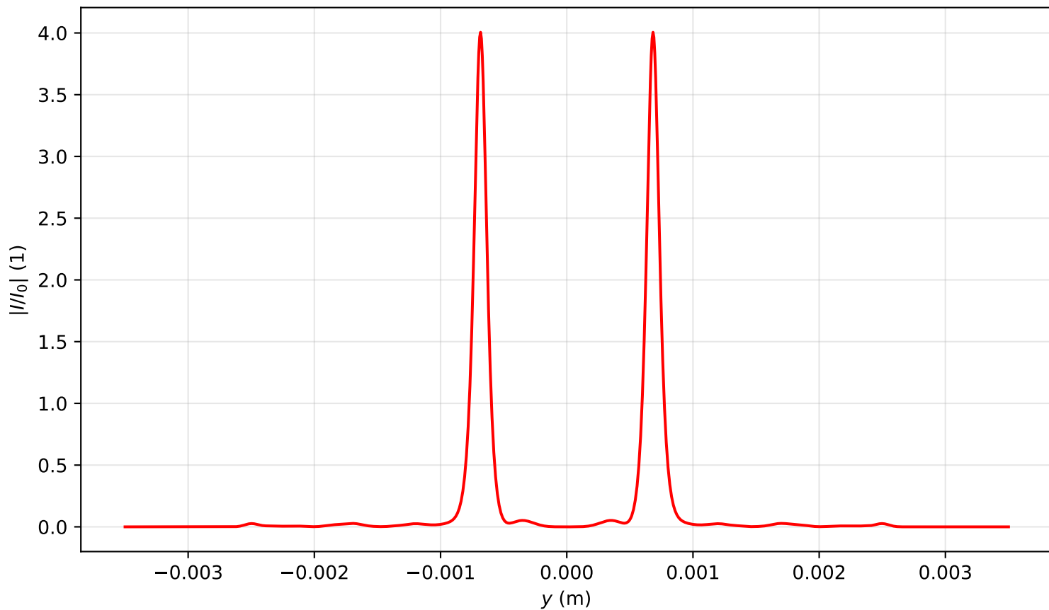
Intensity profile I(x=0, y, z=1.513)/I_0 , P_{in}=19.0P_{cr} , artificial time
