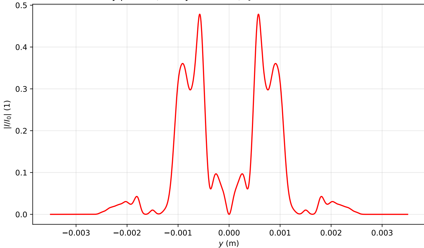
Intensity profile I(x=0, y, z=1.831)/I_0 , P_{in}=19.0P_{cr} , artificial time
