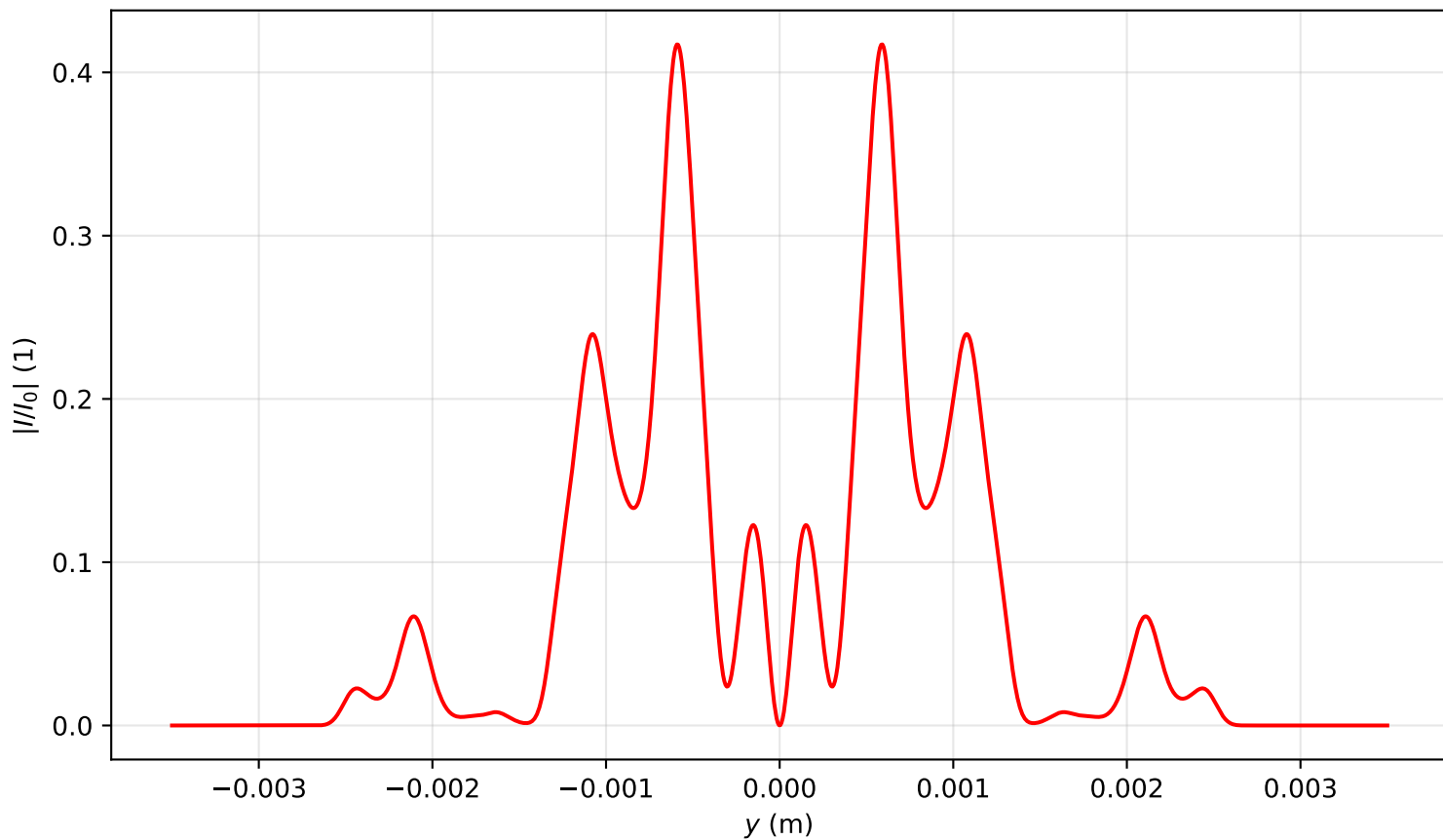
Intensity profile I(x=0, y, z=1.990)/I_0 , P_{in}=19.0P_{cr} , artificial time
