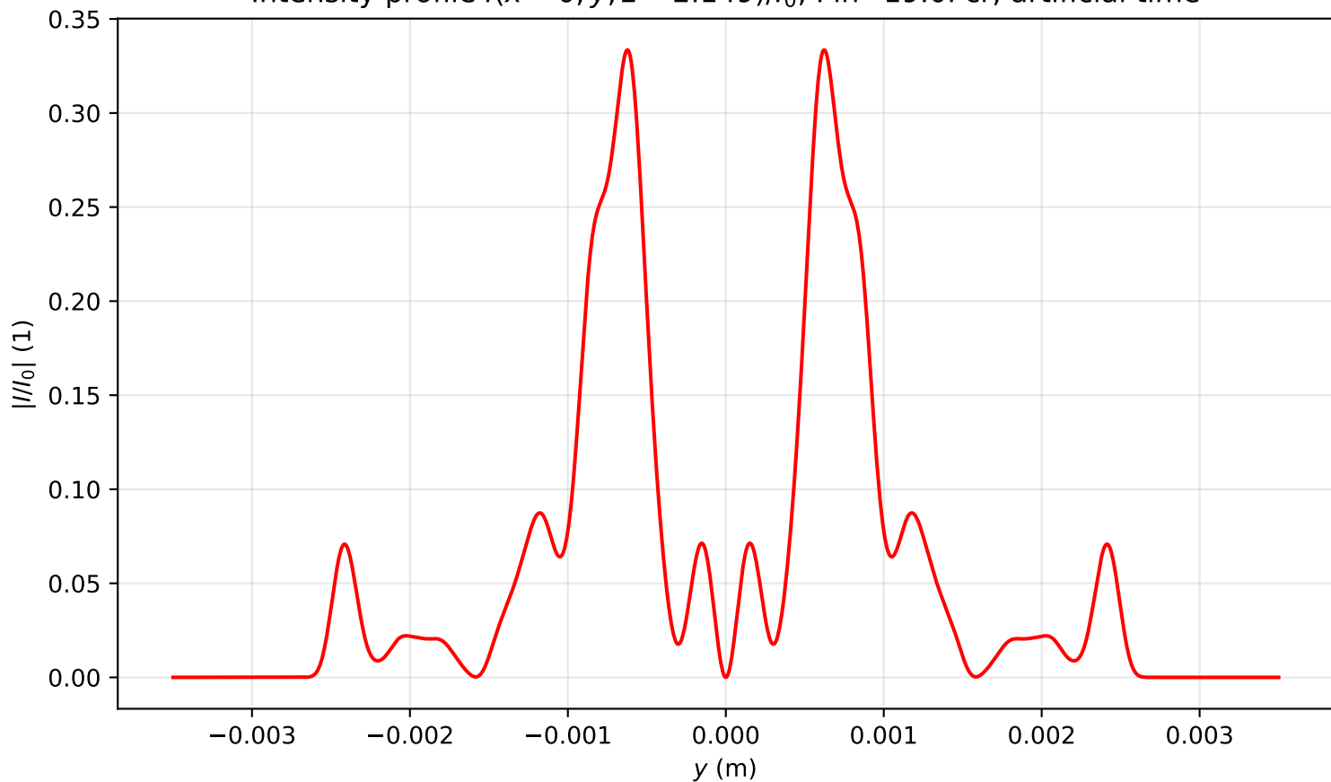
Intensity profile I(x = 0, y, z = 2.149)/I_0 , P_{in}=19.0P_{cr} , artificial time
