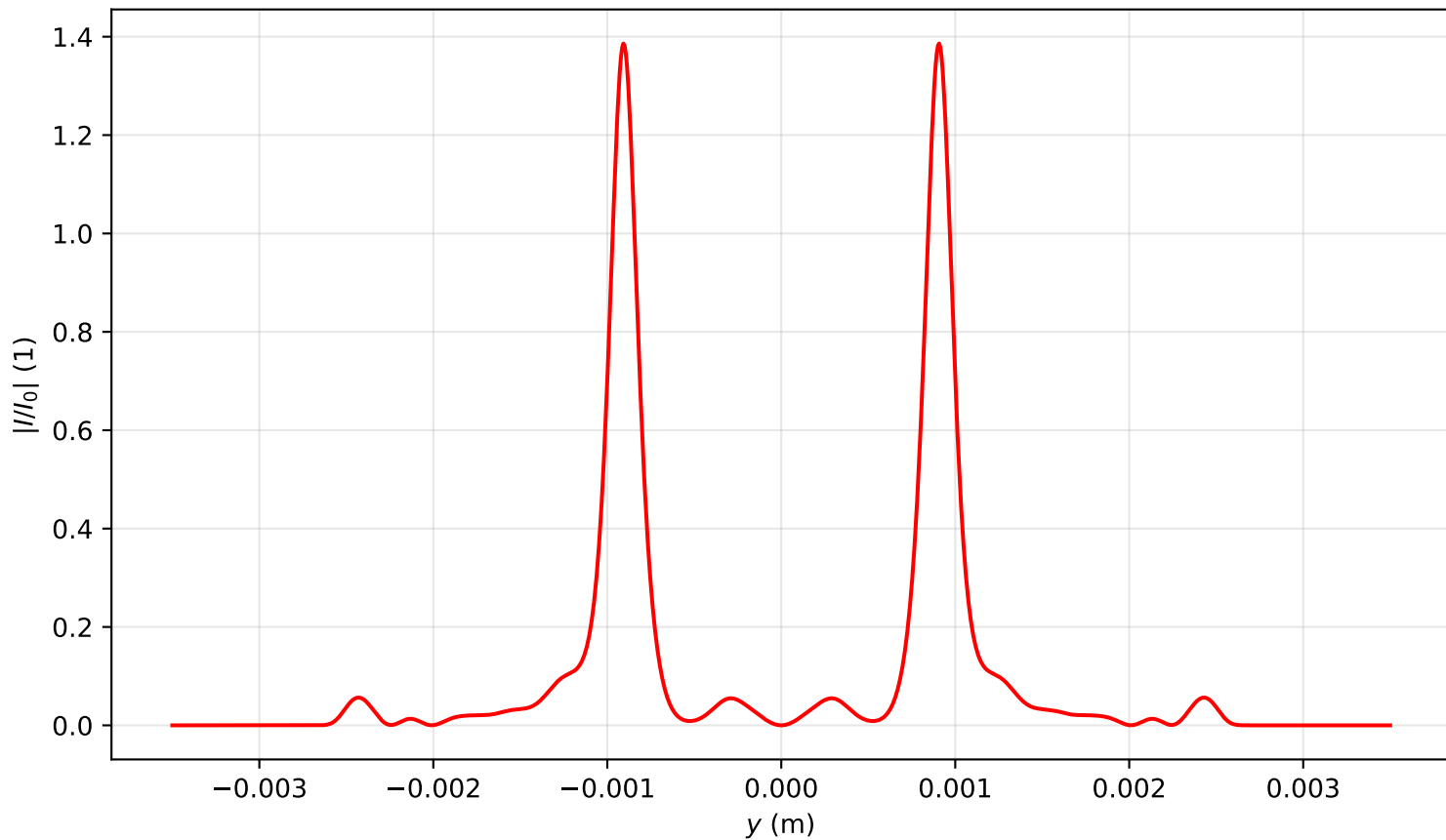
Intensity profile I(x=0, y, z=2.627)/I_0 , P_{in}=19.0P_{cr} , artificial time
