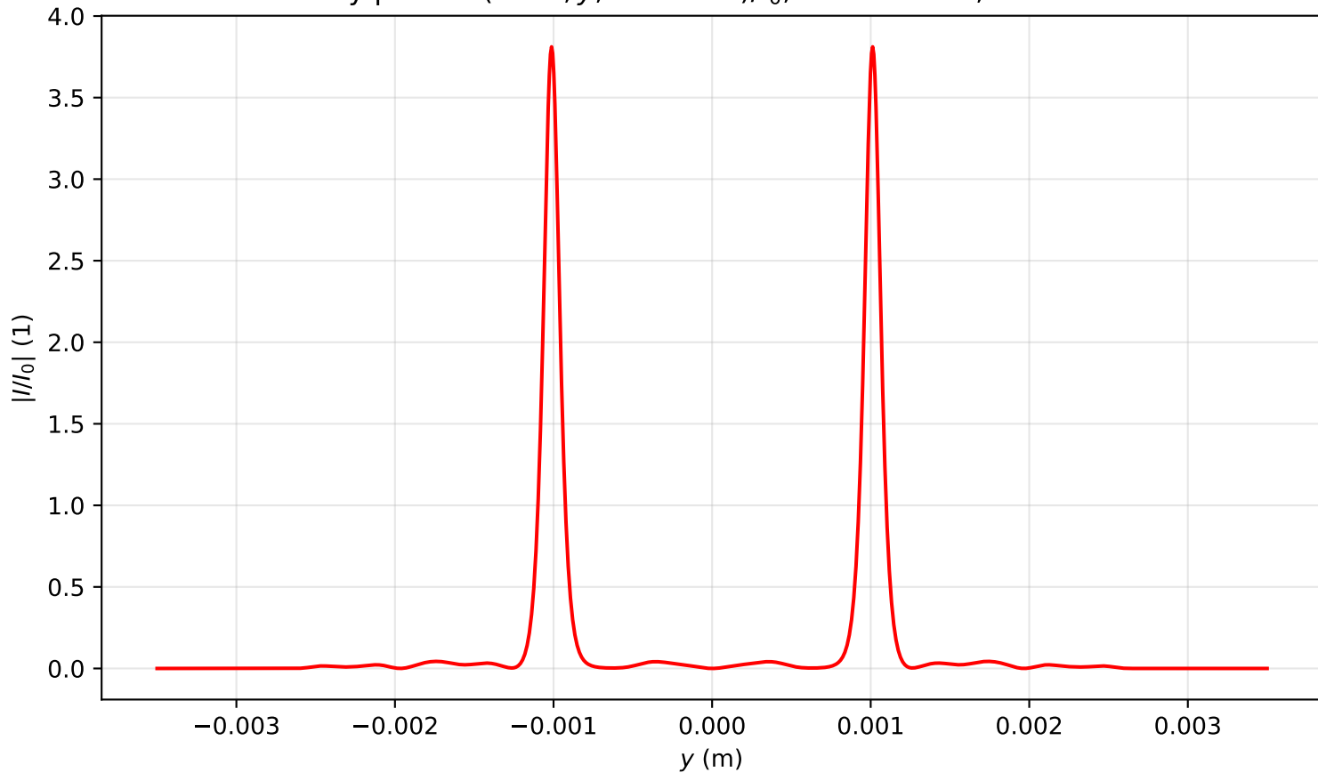
Intensity profile I(x=0, y, z=2.866)/I_0 , P_{in}=19.0P_{cr} , artificial time
