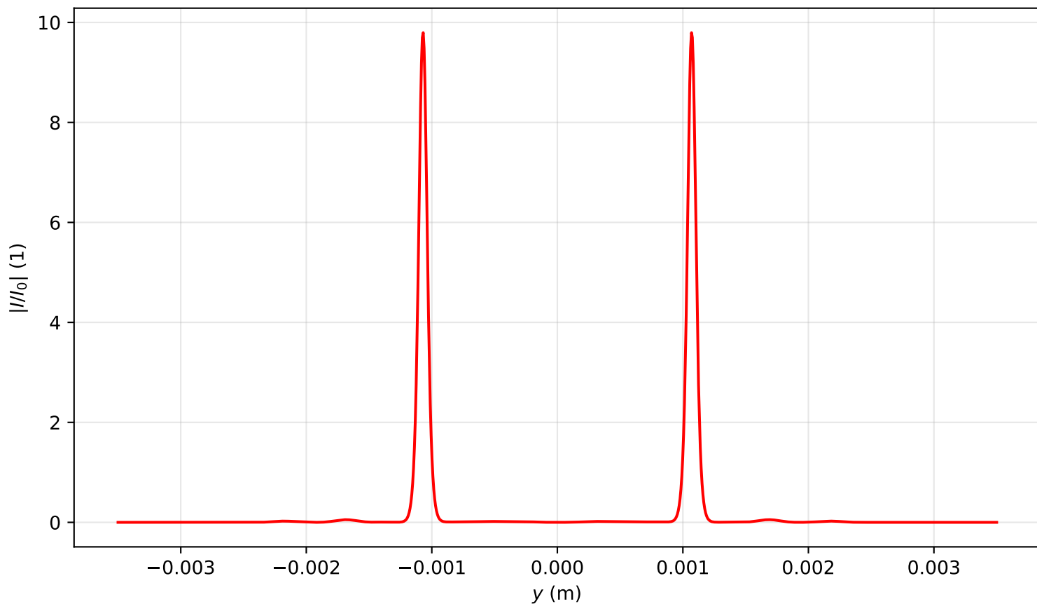
Intensity profile I(x=0, y, z=3.025)/I_0 , P_{in}=19.0P_{cr} , artificial time
