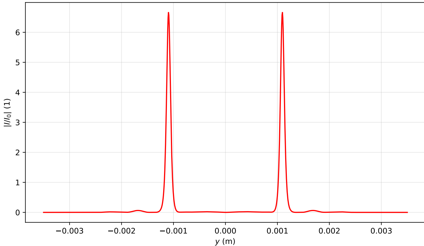
Intensity profile I(x=0, y, z=3.105)/I_0 , P_{in}=19.0\text{Pcr} , artificial time
