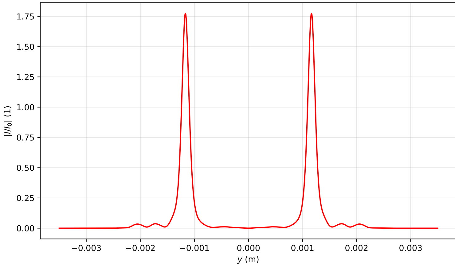
Intensity profile I(x=0, y, z=3.264)/I_0 , P_{in}=19.0\text{Pcr} , artificial time
