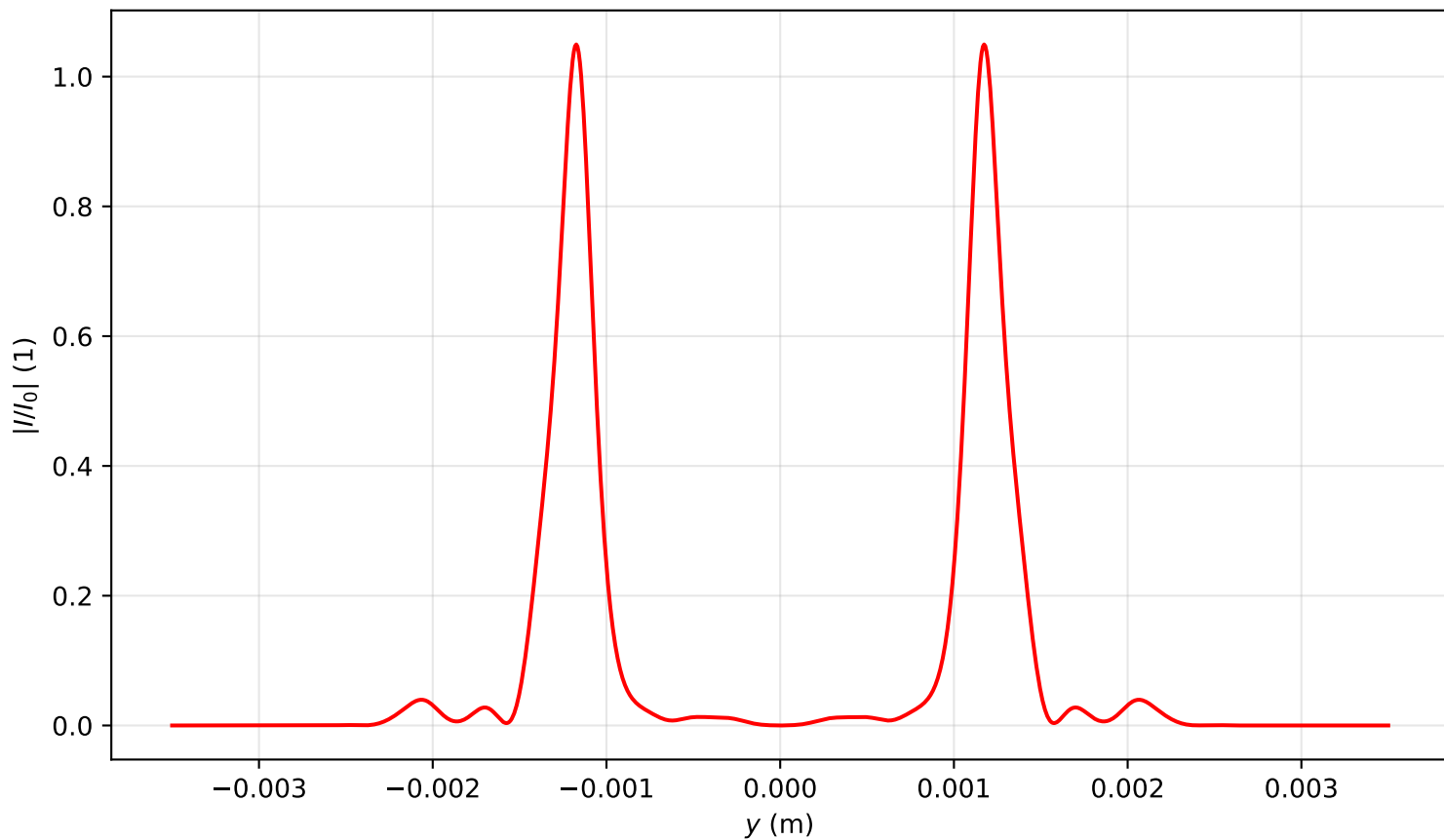
Intensity profile I(x=0, y, z=3.344)/I_0 , P_{in}=19.0P_{cr} , artificial time
