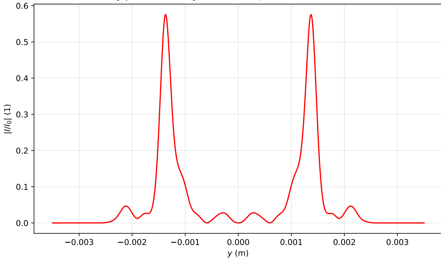
Intensity profile I(x=0, y, z=3.582)/I_0 , P_{in}=19.0\text{Pcr} , artificial time
