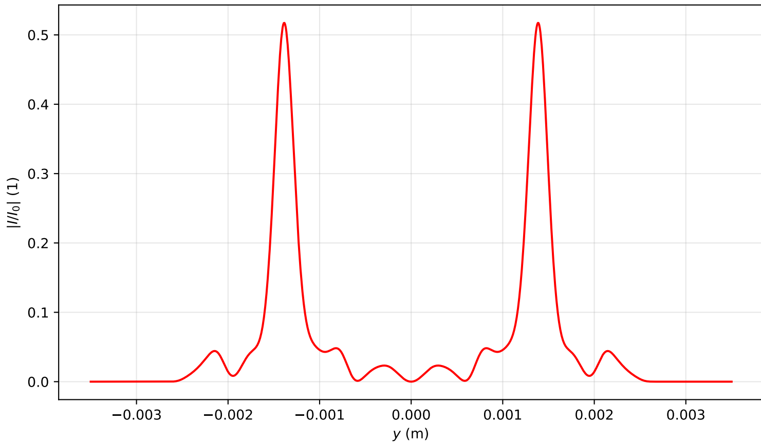
Intensity profile I(x=0, y, z=3.662)/I_0 , P_{in}=19.0P_{cr} , artificial time
