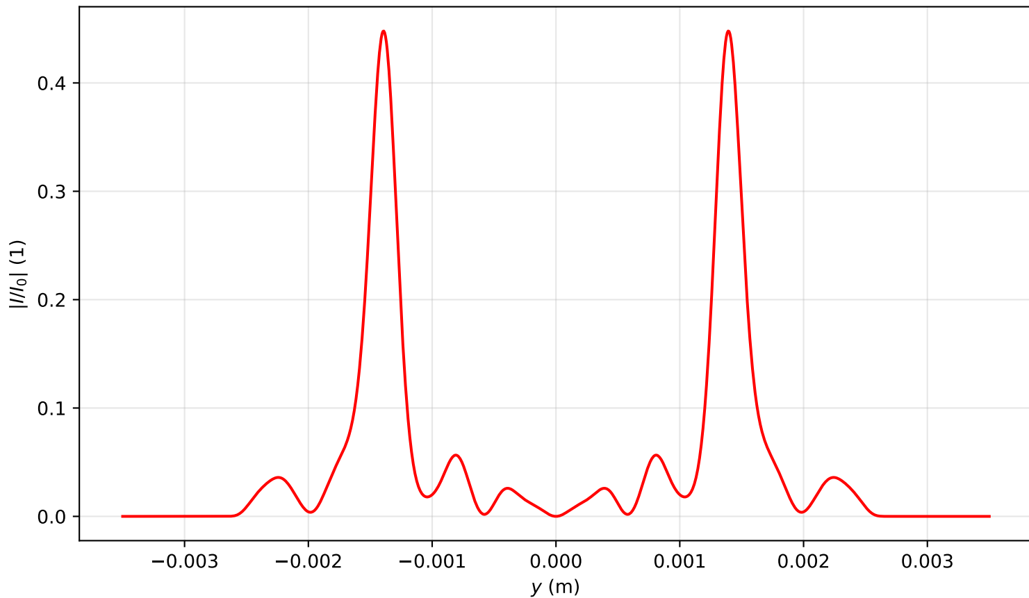
Intensity profile I(x=0, y, z=3.742)/I_0 , P_{in}=19.0\text{Pcr} , artificial time
