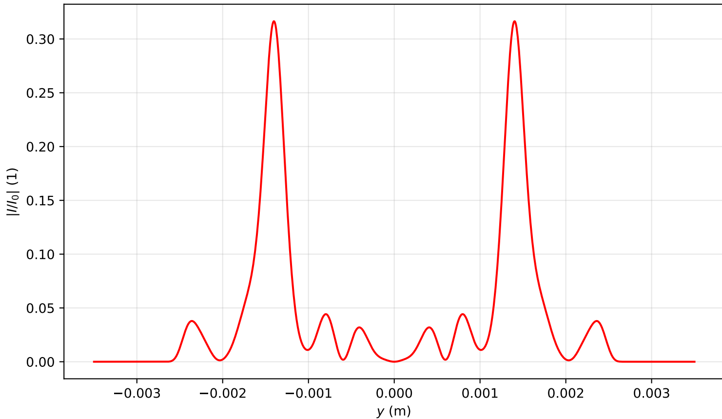
Intensity profile I(x = 0, y, z = 3.821)/I_0 , P_{in}=19.0\text{Pcr} , artificial time
