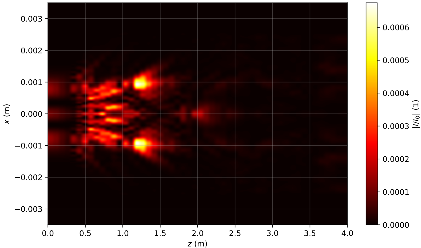
Intensity profile I(x, y = 0, z)/I_0 , P_{in}=19.0P_{cr} , artificial time
