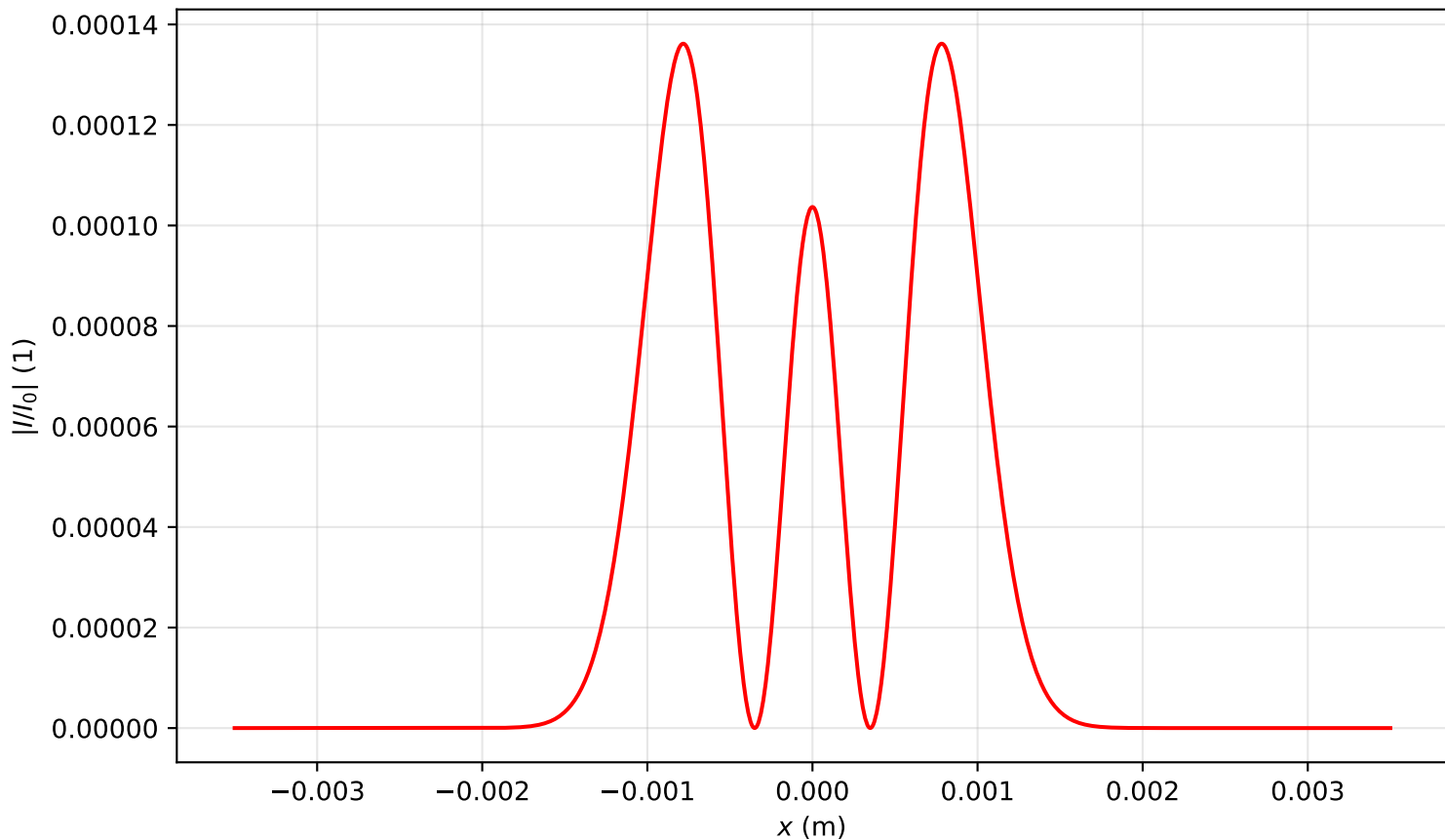
Intensity profile I(x, y = 0, z = 0.000)/I_0 , P_{in}=20.0P_{cr} , artificial time
