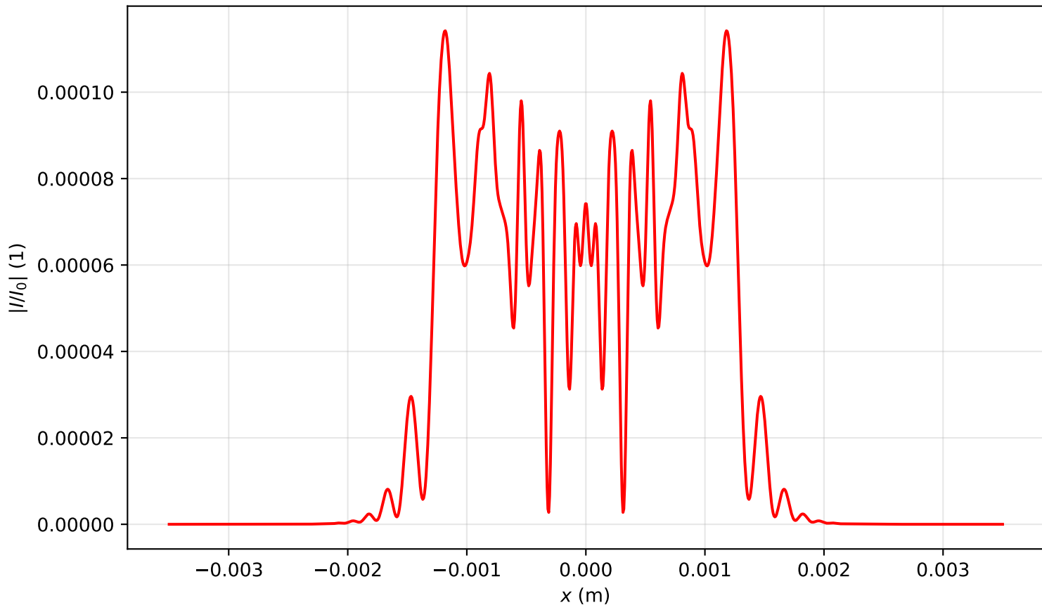
Intensity profile I(x, y = 0, z = 0.398)/I_0 , P_{in}=20.0P_{cr} , artificial time
