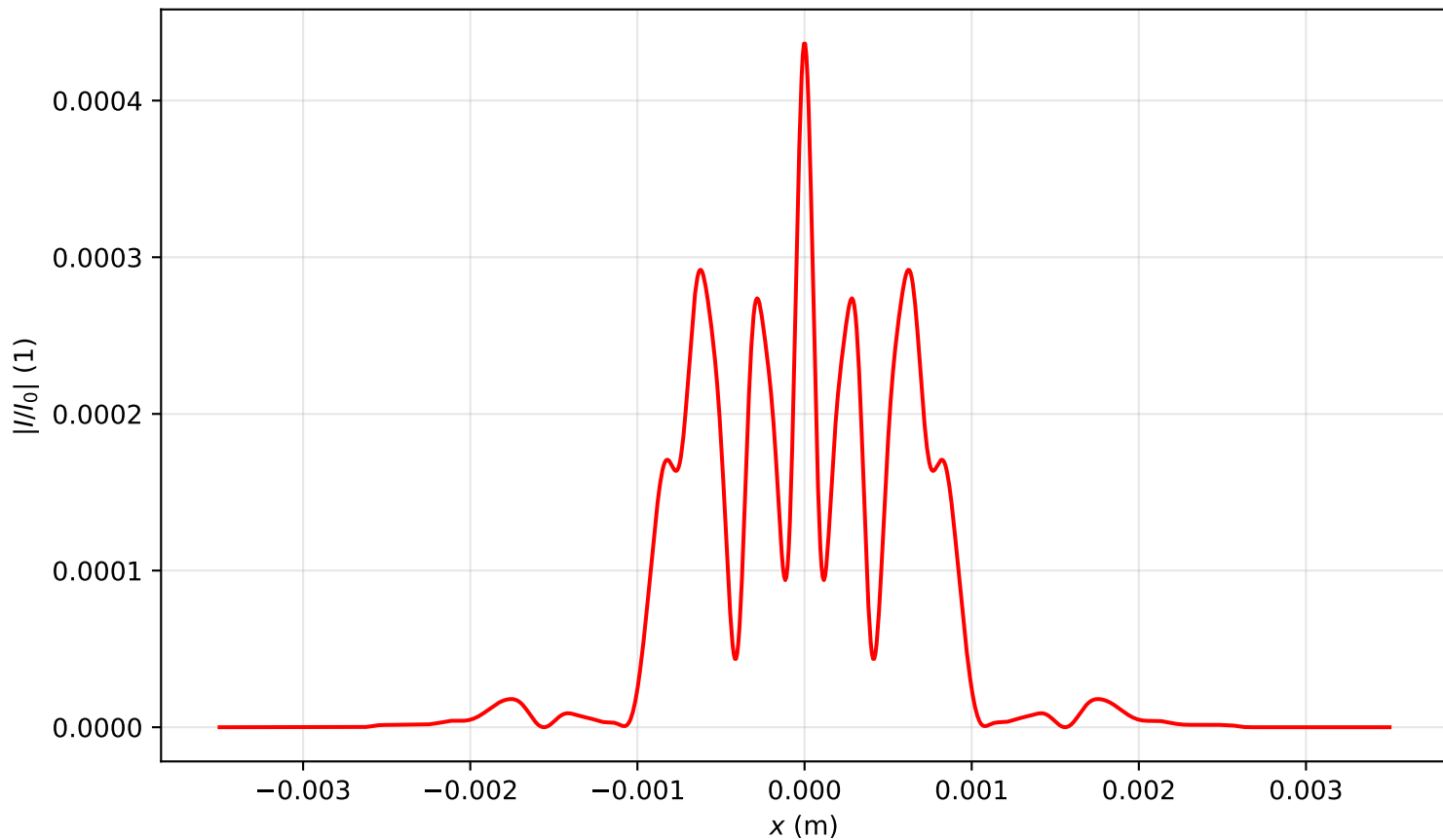
Intensity profile I(x, y = 0, z = 0.716)/I_0 , P_{in}=20.0P_{cr} , artificial time
