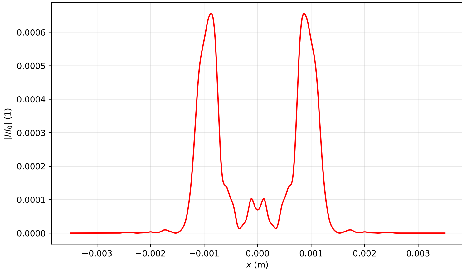
Intensity profile I(x, y = 0, z = 1.194)/I_0 , P_{in}=20.0\text{Pcr} , artificial time
