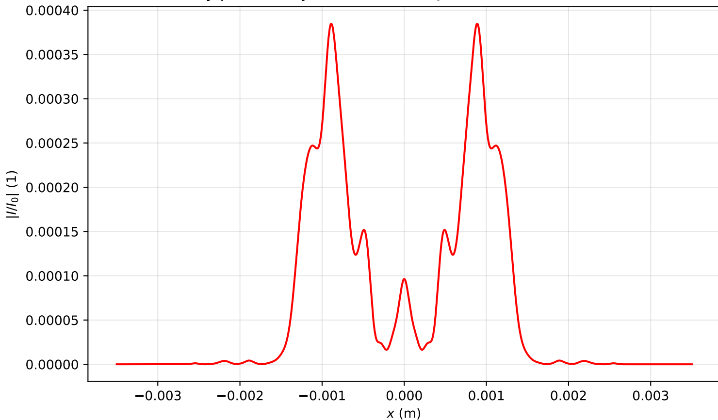
Intensity profile I(x, y = 0, z = 1.274)/I_0 , P_{in}=20.0\text{Pcr} , artificial time
