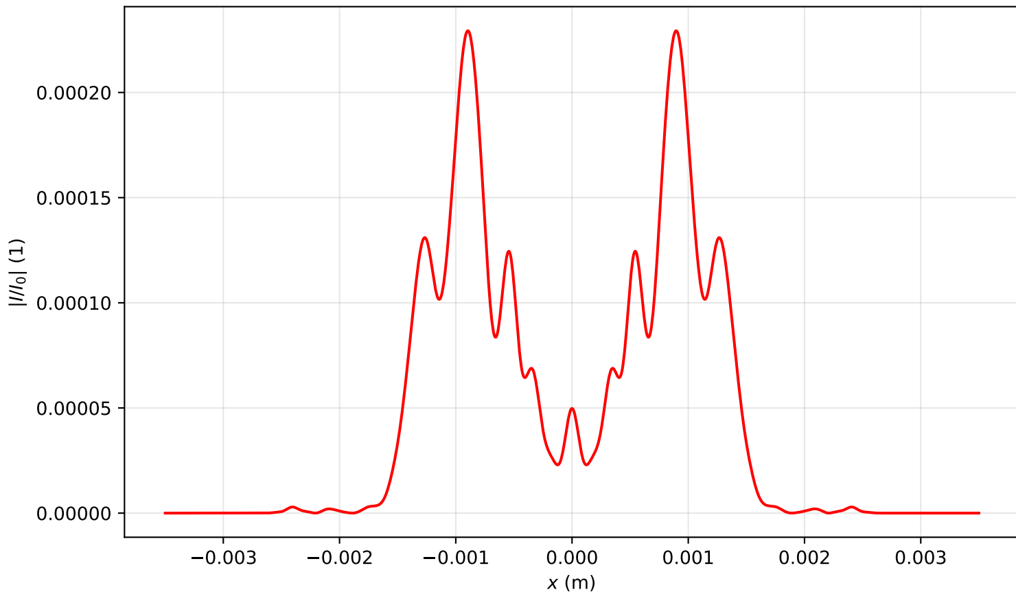
Intensity profile I(x, y = 0, z = 1.353)/I_0 , P_{in}=20.0P_{cr} , artificial time
