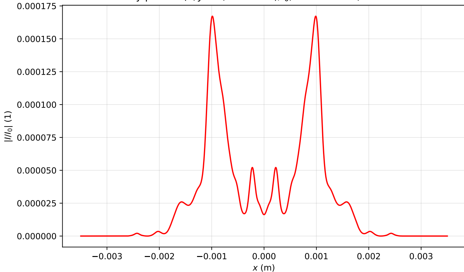
Intensity profile I(x, y = 0, z = 1.513)/I_0 , P_{in}=20.0P_{cr} , artificial time
