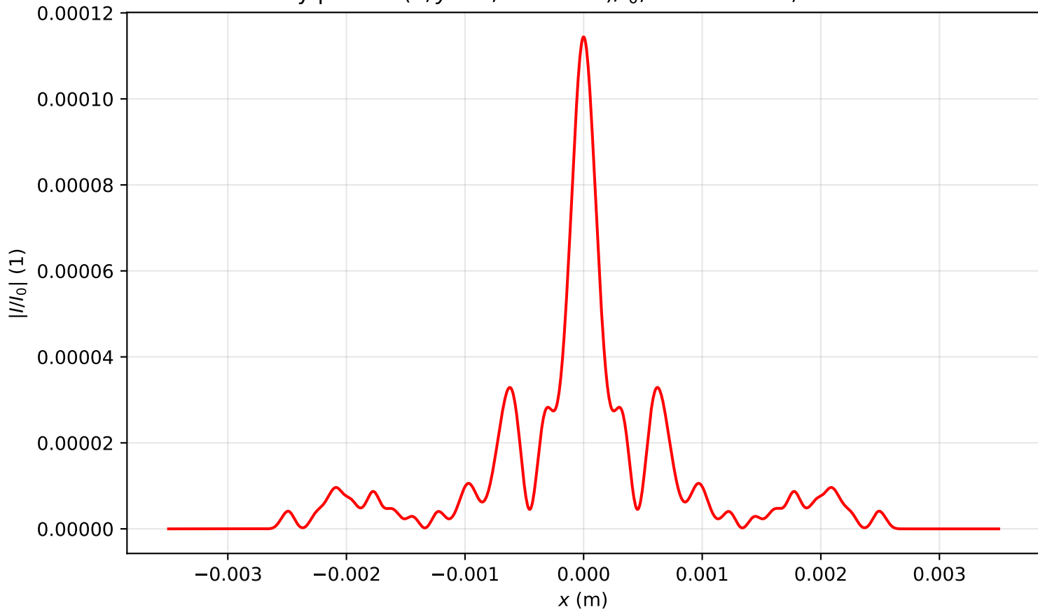
Intensity profile I(x, y = 0, z = 1.831)/I_0 , P_{in}=20.0P_{cr} , artificial time
