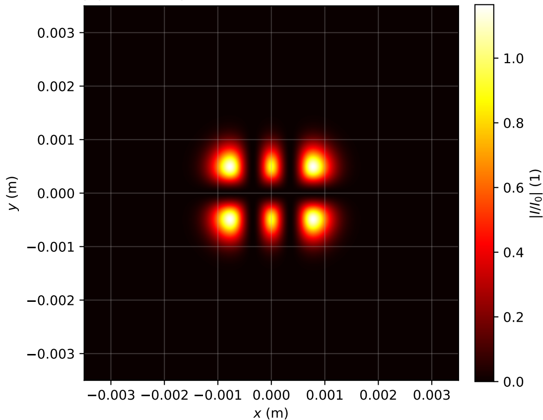
Intensity profile I(x, y, z = 0.080)/I_0 , P_{in}=20.0\text{Pcr} , artificial time
