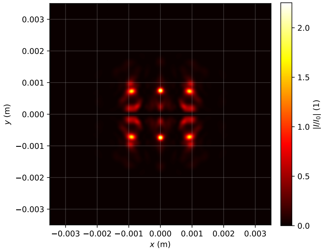
Intensity profile I(x, y, z = 1.115)/I_0 , P_{in}=20.0\text{Pcr} , artificial time
