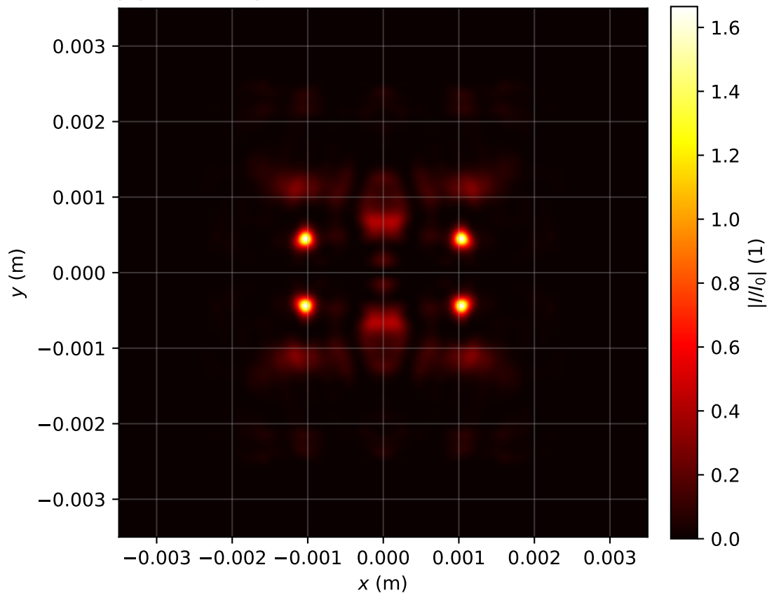
Intensity profile I(x, y, z = 1.990)/I_0 , P_{in}=20.0\text{Pcr} , artificial time
