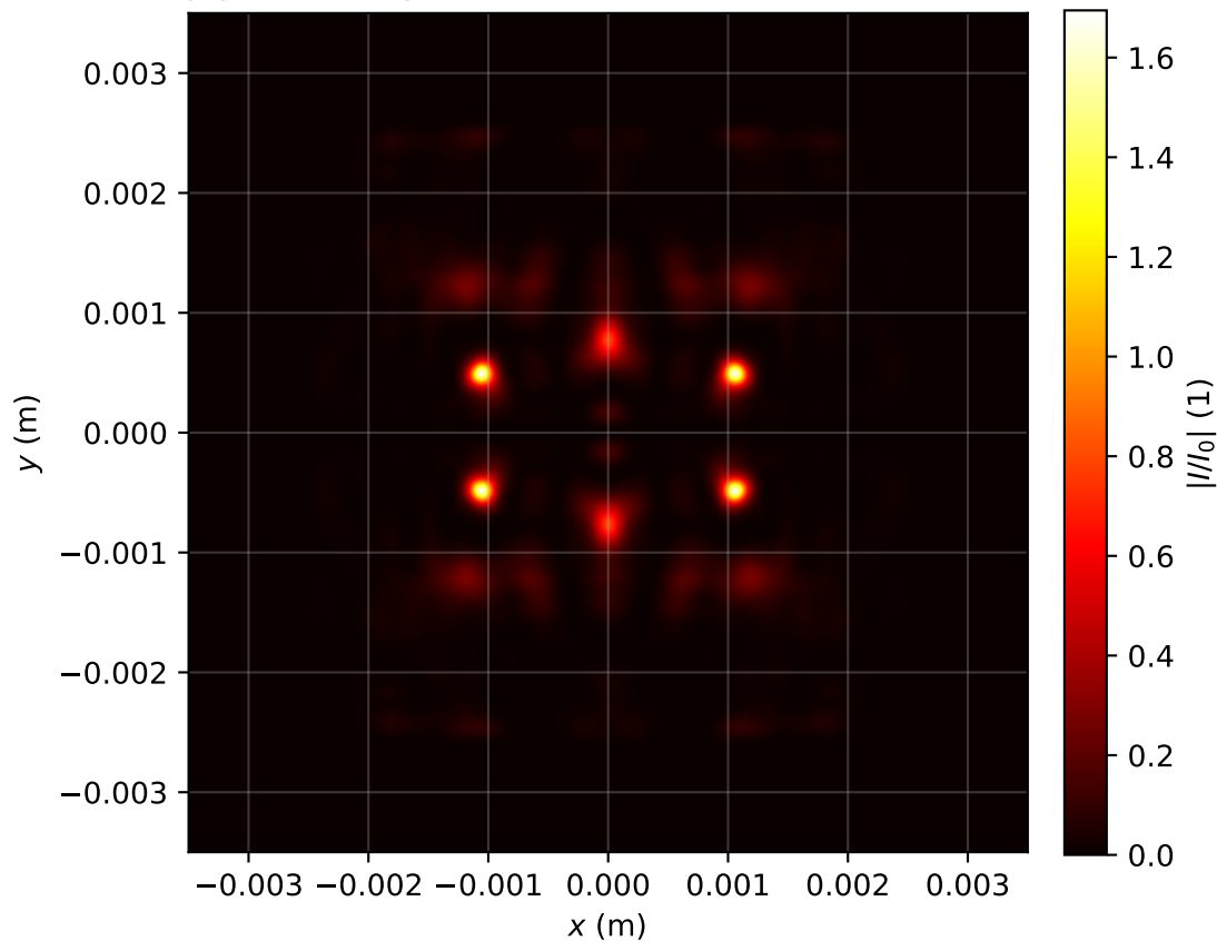
Intensity profile I(x, y, z = 2.149)/I_0 , P_{in}=20.0\text{Pcr} , artificial time
