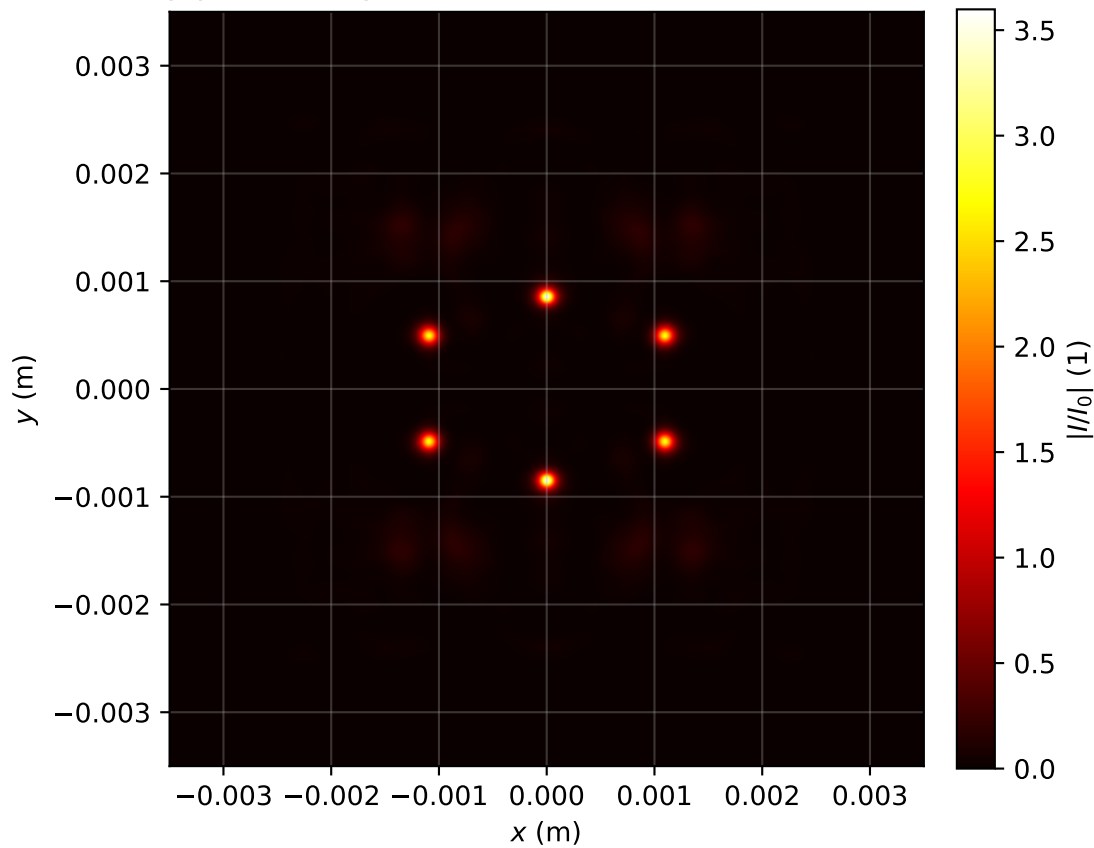
Intensity profile I(x, y, z = 2.468)/I_0 , P_{in}=20.0\text{Pcr} , artificial time
