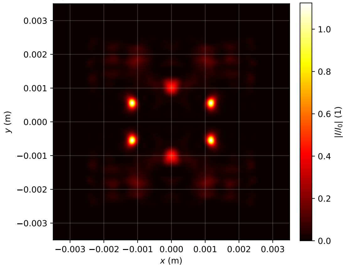
Intensity profile I(x, y, z = 2.946)/I_0 , P_{in}=20.0\text{Pcr} , artificial time
