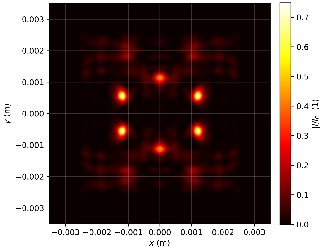
Intensity profile I(x, y, z = 3.105)/I_0 , P_{in}=20.0\text{Pcr} , artificial time
