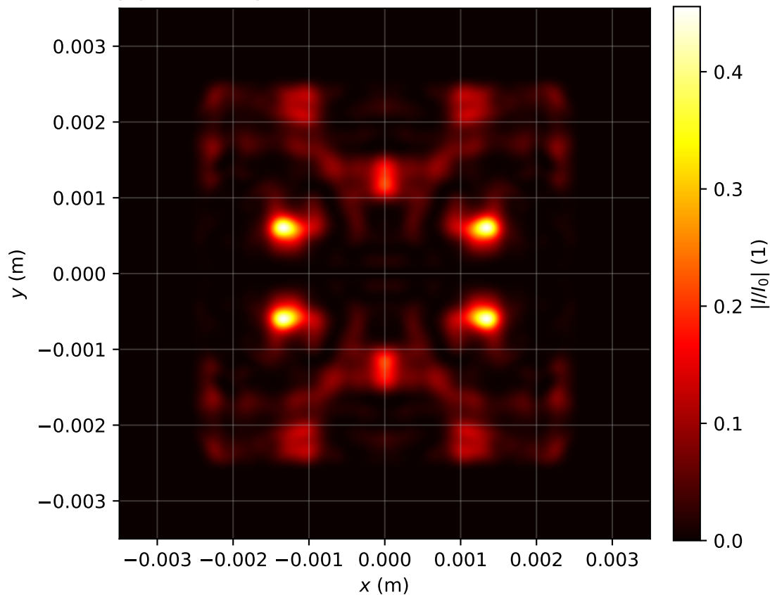
Intensity profile I(x, y, z = 3.344)/I_0 , P_{in}=20.0\text{Pcr} , artificial time
