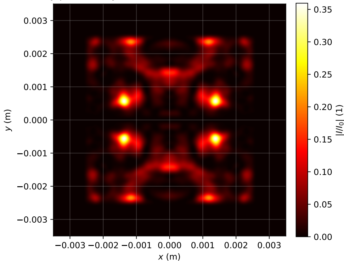
Intensity profile I(x, y, z = 3.503)/I_0 , P_{in}=20.0P_{cr} , artificial time
