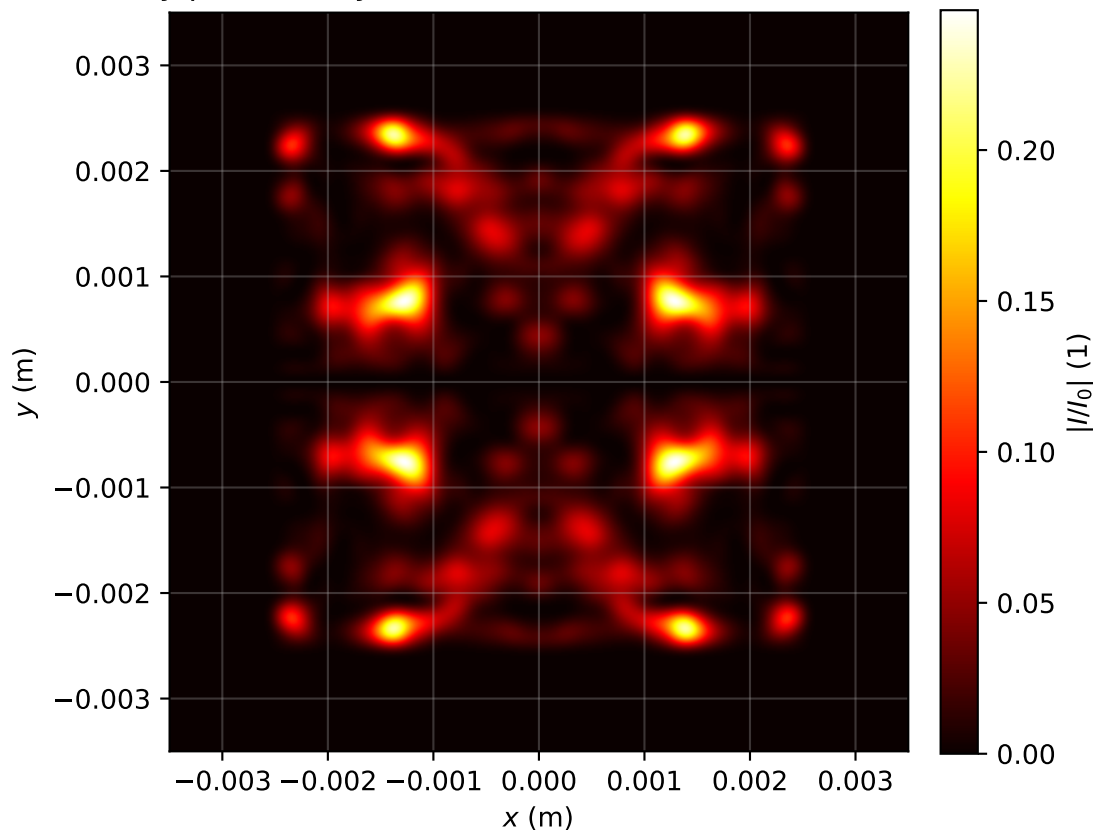
Intensity profile I(x, y, z = 3.981)/I_0 , P_{in}=20.0\text{Pcr} , artificial time
