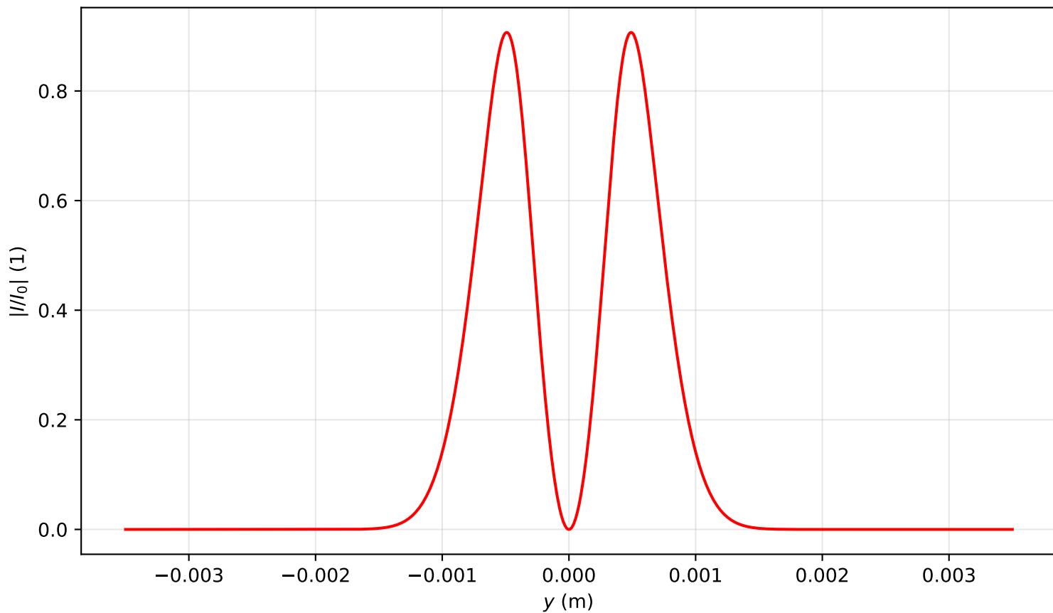
Intensity profile I(x=0, y, z=0.080)/I_0 , P_{in}=20.0P_{cr} , artificial time
