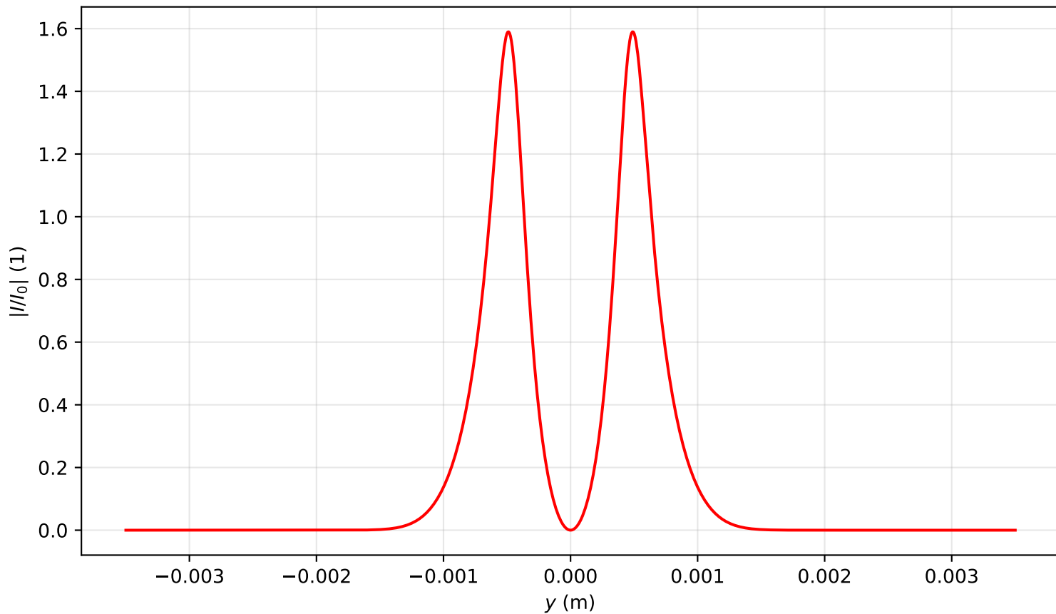
Intensity profile I(x=0, y, z=0.159)/I_0 , P_{in}=20.0P_{cr} , artificial time
