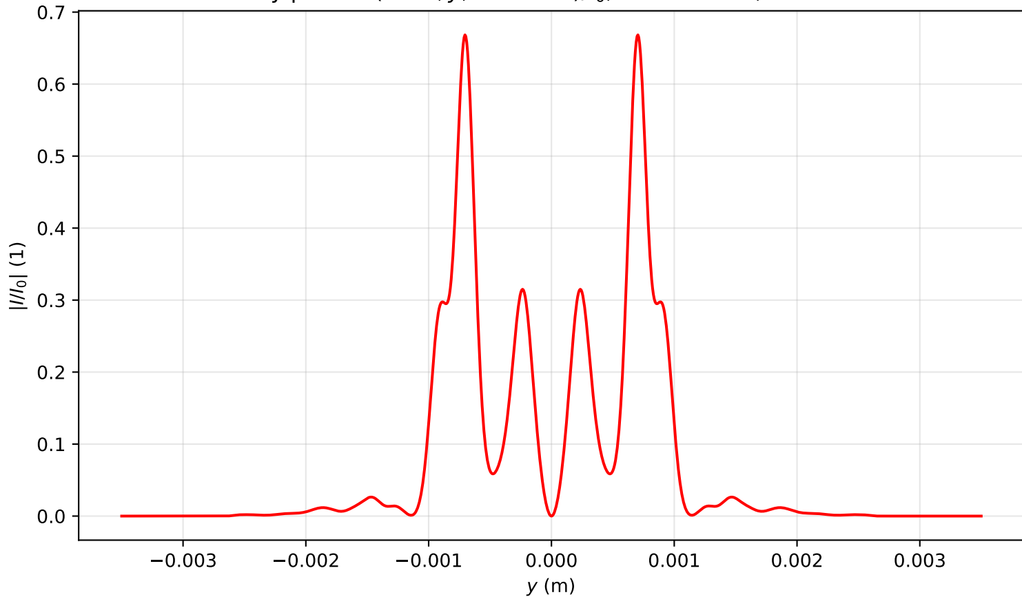
Intensity profile I(x=0, y, z=0.796)/I_0 , P_{in}=20.0P_{cr} , artificial time
