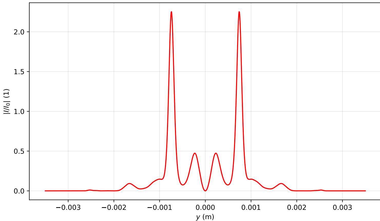
Intensity profile I(x=0, y, z=1.115)/I_0 , P_{in}=20.0\text{Pcr} , artificial time
