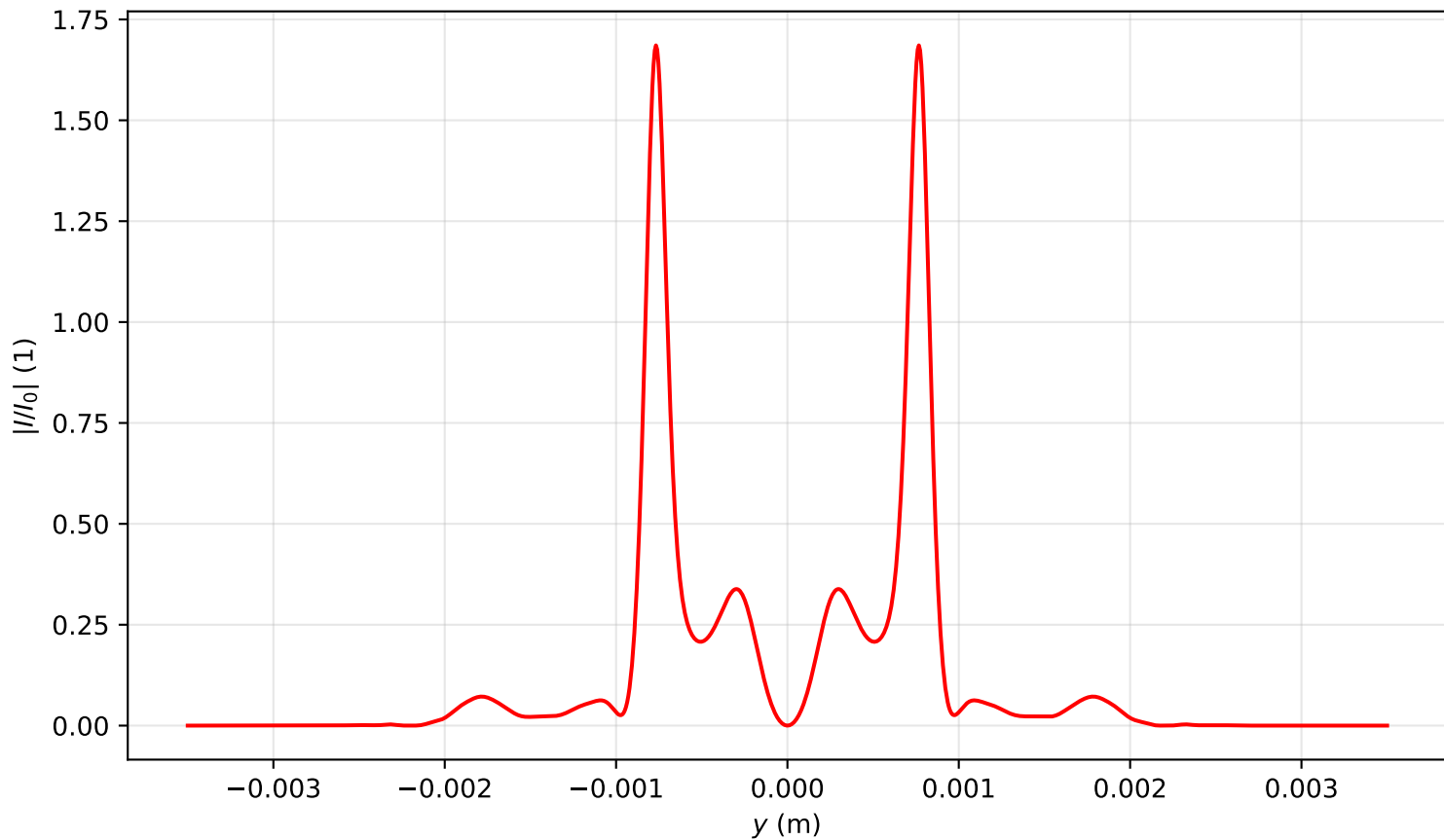
Intensity profile I(x=0, y, z=1.194)/I_0 , P_{in}=20.0\text{Pcr} , artificial time
