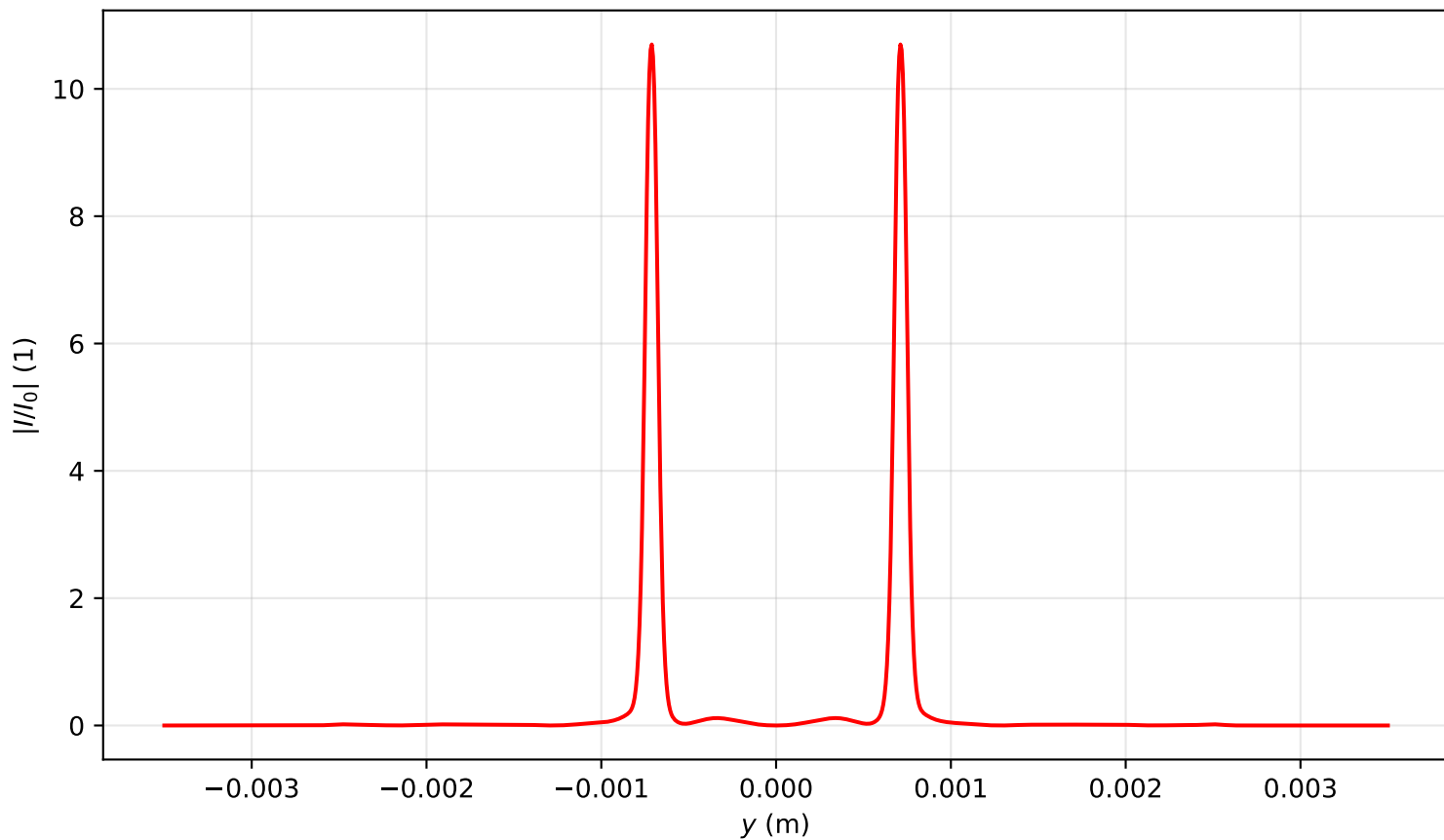
Intensity profile I(x = 0, y, z = 1.513)/I_0 , \text{Pin}=20.0\text{Pcr} , artificial time
