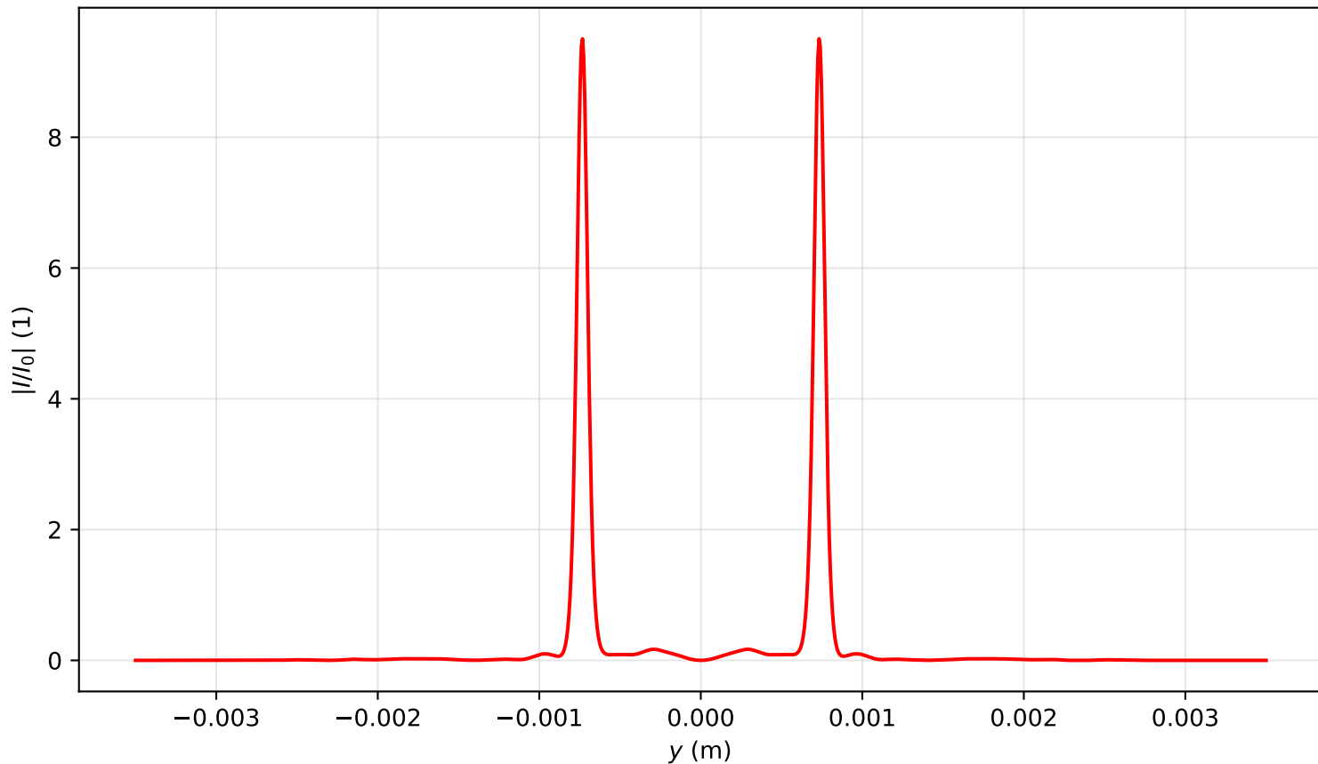
Intensity profile I(x=0, y, z=1.592)/I_0 , P_{in}=20.0P_{cr} , artificial time
