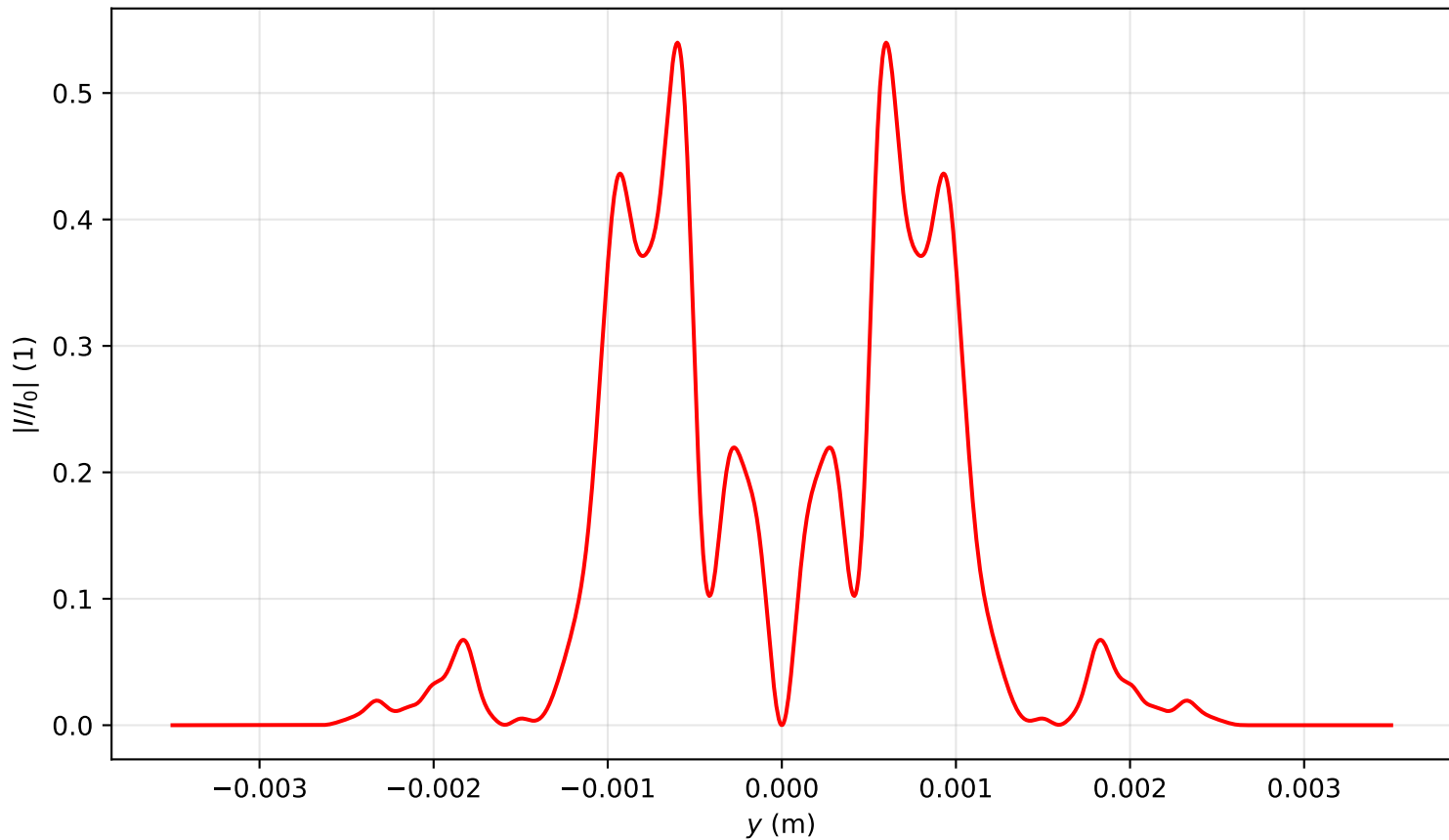
Intensity profile I(x=0, y, z=1.751)/I_0 , P_{in}=20.0\text{Pcr} , artificial time
