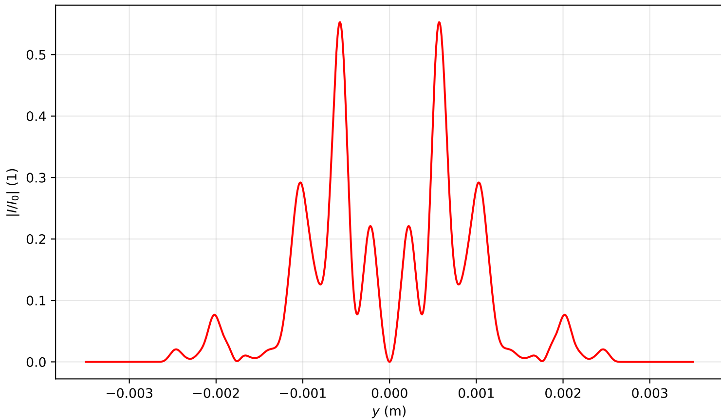
Intensity profile I(x=0, y, z=1.831)/I_0 , P_{in}=20.0\text{Pcr} , artificial time
