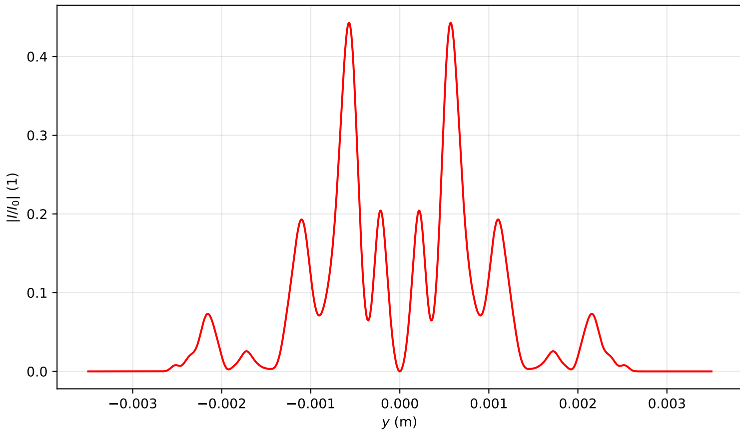
Intensity profile I(x=0, y, z=1.911)/I_0 , P_{in}=20.0P_{cr} , artificial time
