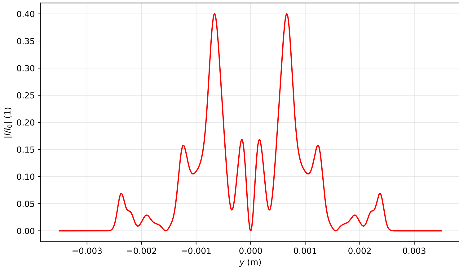
Intensity profile I(x = 0, y, z = 1.990)/I_0 , P_{in}=20.0P_{cr} , artificial time
