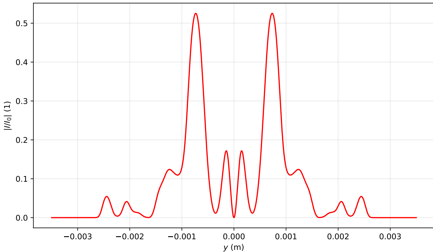
Intensity profile I(x=0, y, z=2.070)/I_0 , P_{in}=20.0\text{Pcr} , artificial time
