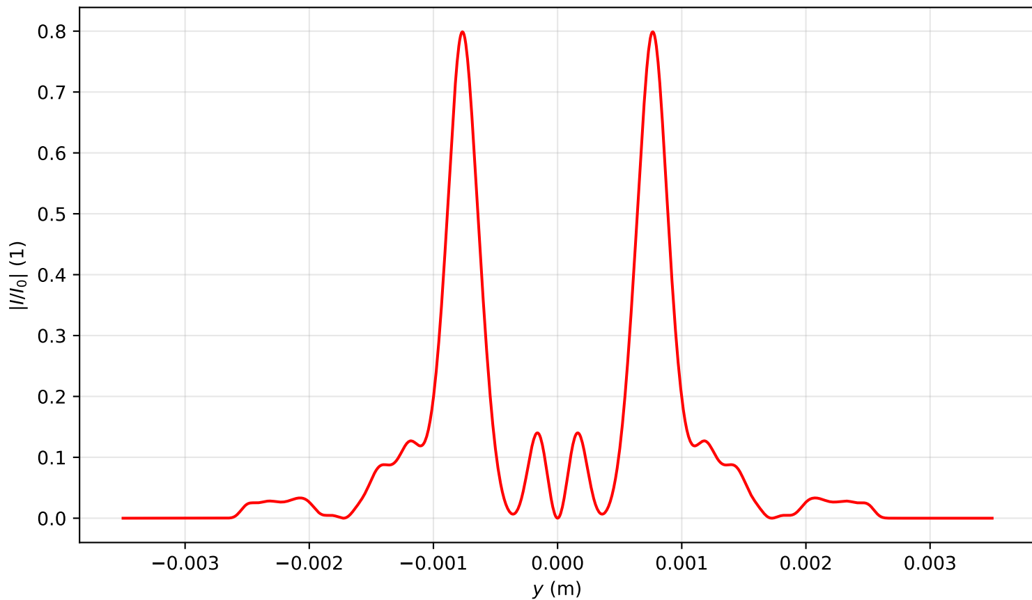
Intensity profile I(x=0, y, z=2.149)/I_0 , P_{in}=20.0P_{cr} , artificial time
