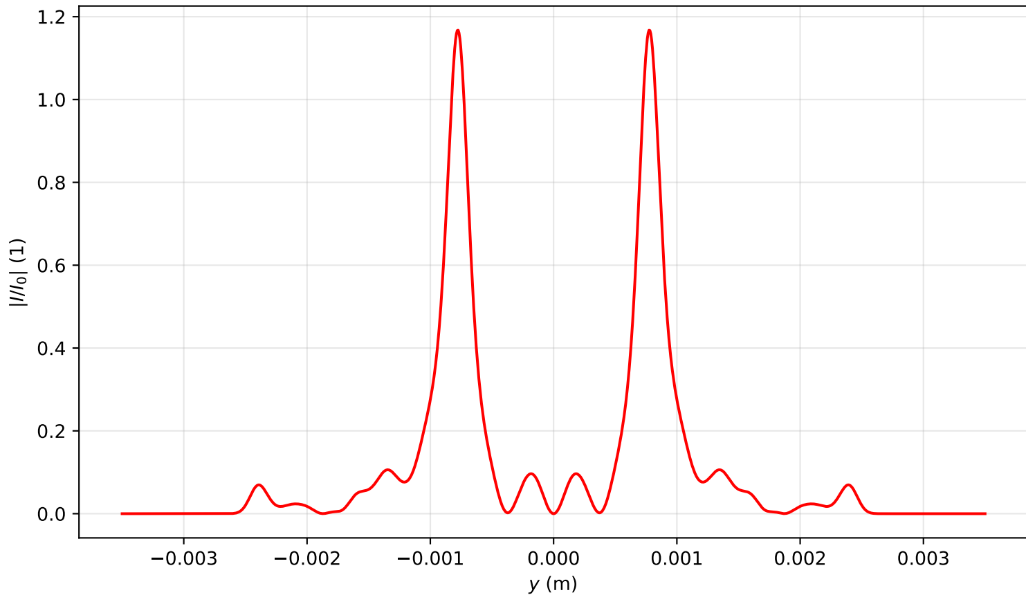
Intensity profile I(x=0, y, z=2.229)/I_0 , P_{in}=20.0\text{Pcr} , artificial time
