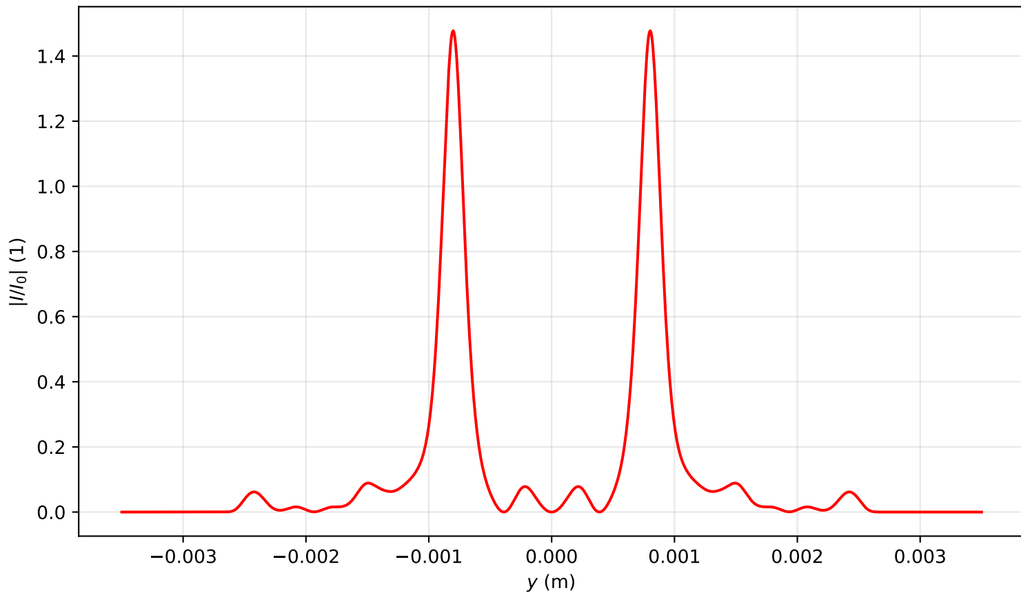
Intensity profile I(x=0, y, z=2.309)/I_0 , P_{in}=20.0\text{Pcr} , artificial time
