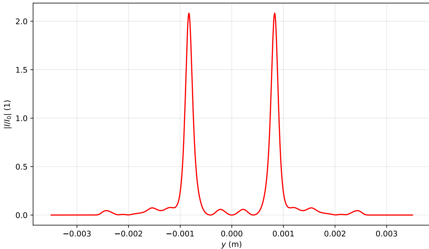
Intensity profile I(x=0, y, z=2.388)/I_0 , P_{in}=20.0\text{Pcr} , artificial time
